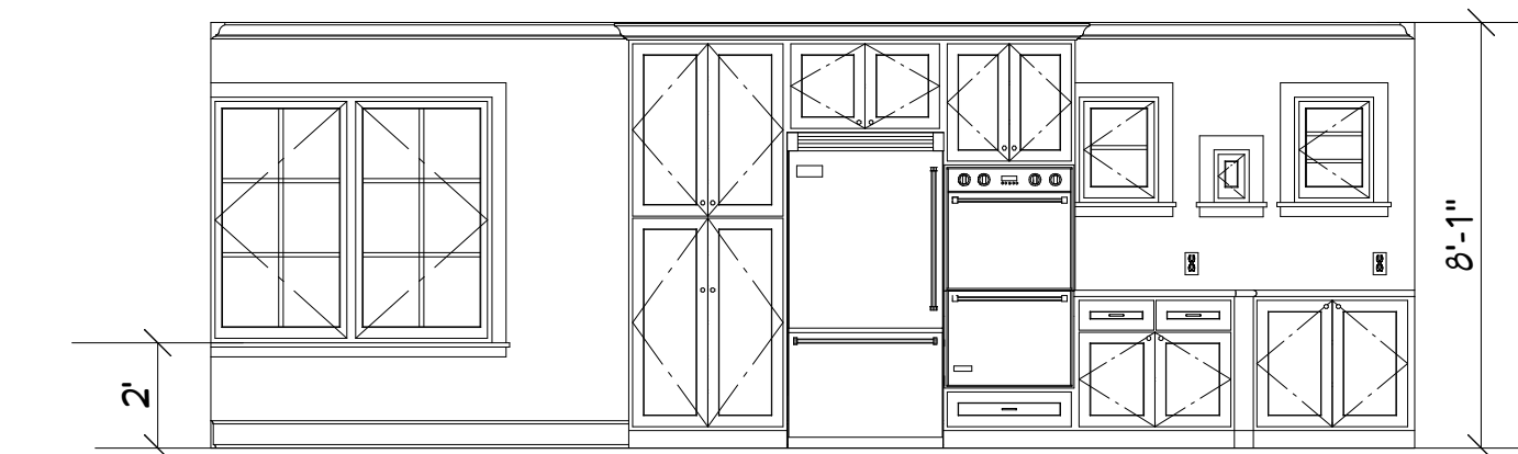
CROSS SECTION "A" SCALE: 1/4" = 1'-0"
